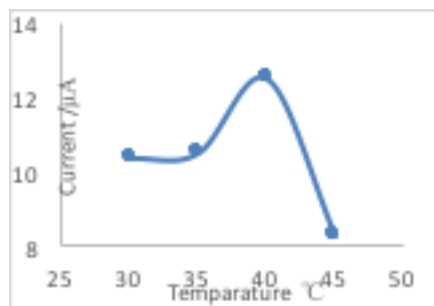
Figure 4. Calibration curve of temperature (Sodyum Acetat buffer, pH 6.0, 50 mM).
