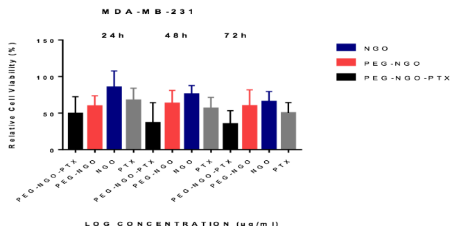
Figure 3. Cytotoxicity effect of NGO, NGO-PEG, NGO-PEG-PTX and PTX drugs on MDA-MB-231 cell line.
