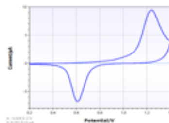
Figure 1. The cyclic voltammograms of the biosensor at different stages in a potential range of (+0.2)-(+1.4) V at sodium acetat buffer solution at a scan rate of 0.6 Vs -1 . According to the figure 1 redox peak appeared in the cyclic voltammogram of the Au electrode.
