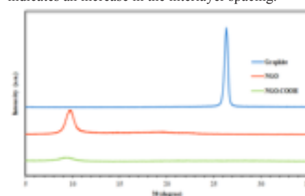
Figure 1. The XRD patterns of graphite, NGO and NGO-COOH.
